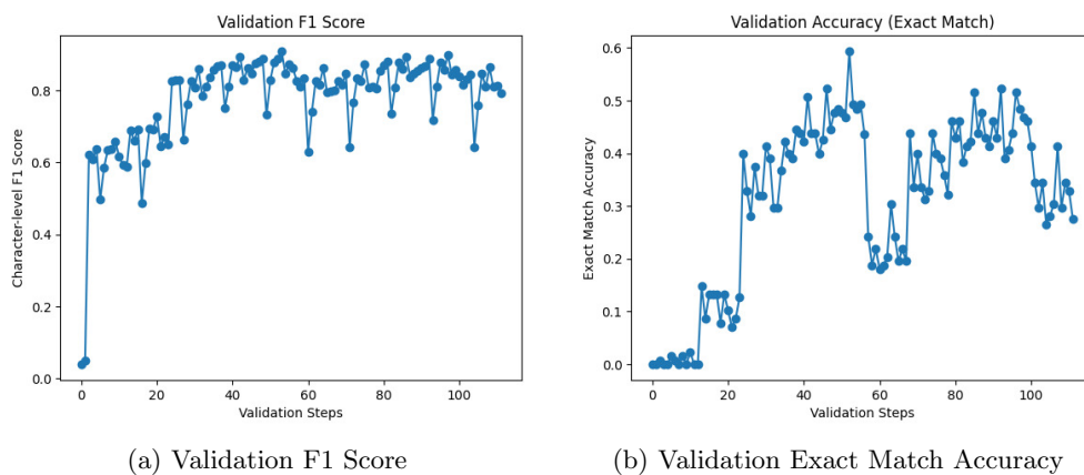
Fig. 5: Validation performance metrics for the Sandhi splitting model.
