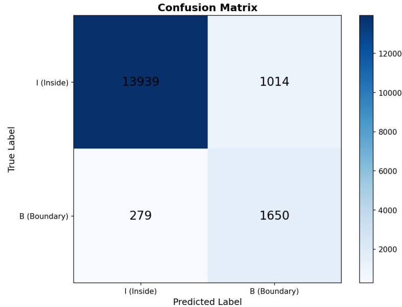
Fig. 7: Boundary Detection Confusion Matrix
